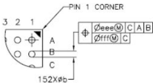
DETAIL B(2:1)
