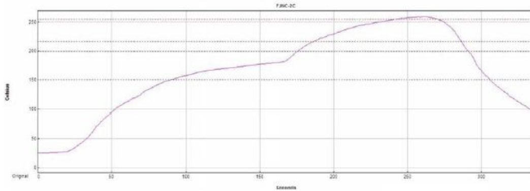
(Figure 6-1 Recommended Reflow Profile)
